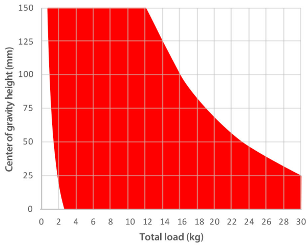
Payload Diagram FSB 14T Mk II
