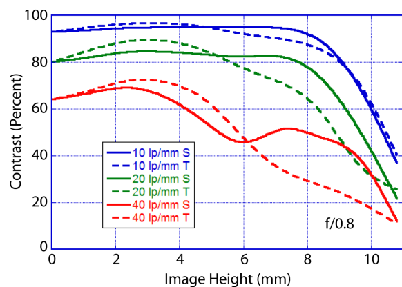
Figure 2: MTF at 10, 20, and 40 lp/mm for f/0.80
