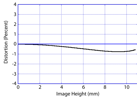
Figure 6: Distortion
