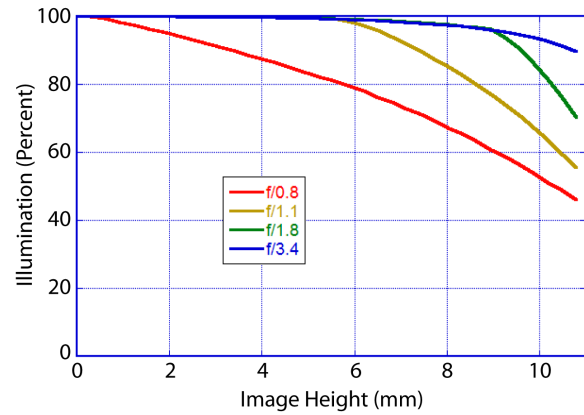
Figure 5: Relative illumination
