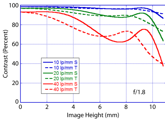
Figure 4: MTF at 10, 20, and 40 lp/mm for f/1.8
