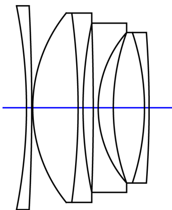
Figure 1: Speed Booster XL 0.64x design layout
