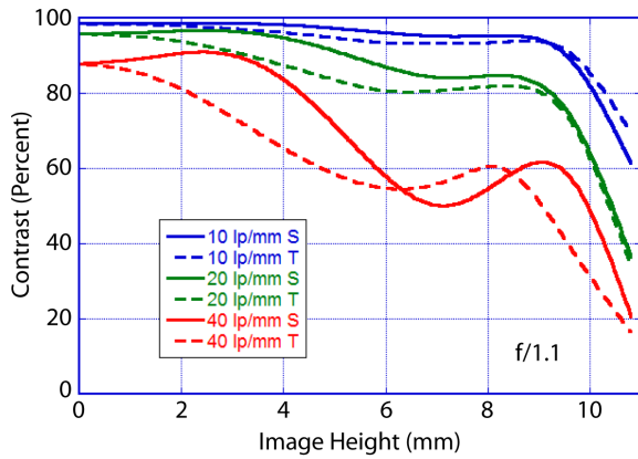
Figure 3: MTF at 10, 20 and 40 lp/mm for f/1.1
